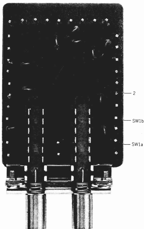
FIG. 12 PHOTO OF TAPE P.C. BOARD (96-5001) BLOCK
