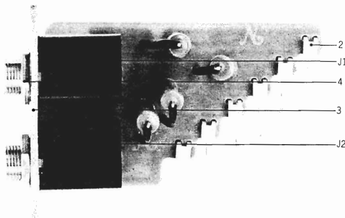
FIG. 10 PHOTO OF HP P.C. BOARD (98-5012) BLOCK
